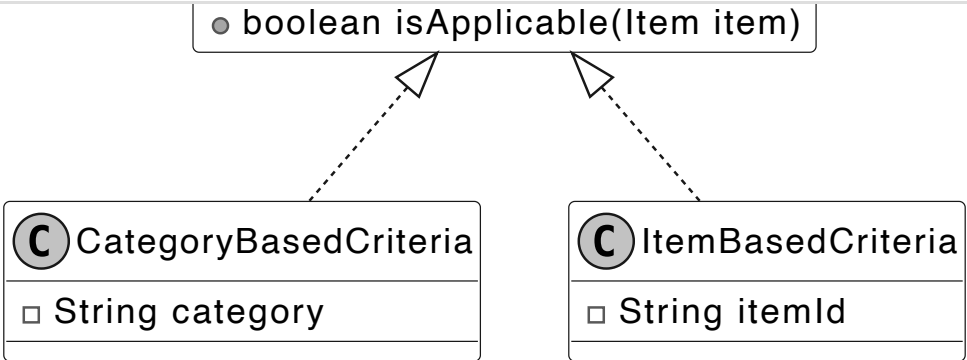
DiscountCriteria interface and concrete classes
