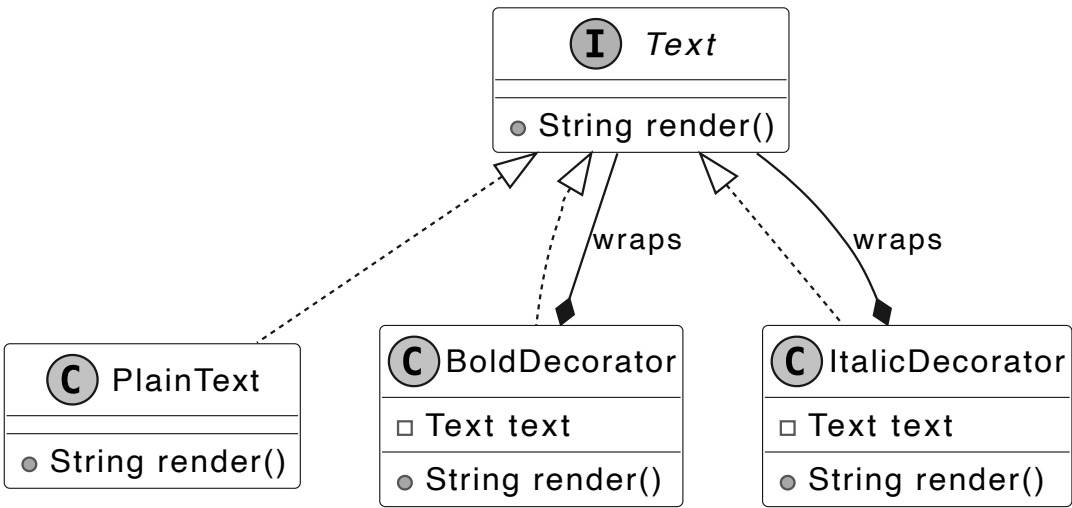
Text interface and concrete classes
